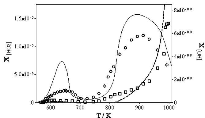
Fig. 4. Estimated •OH (□) and •HO 2 (○) radical mole fractions obtained from calibrated LIF signals compared with predictions using a detailed kinetic model (18).
