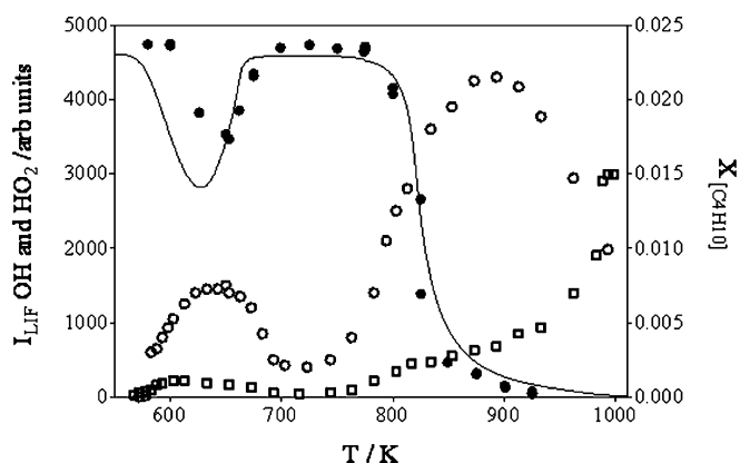
Fig. 3. •OH (□) and •HO 2 (○) radical fluorescence intensity signals (in arbitrary units; Left y axis) as a function of temperature, as well as experimental (●) and predicted (black line; see SI Text for details) n -butane mole fraction profiles (18) (Right y axis).
